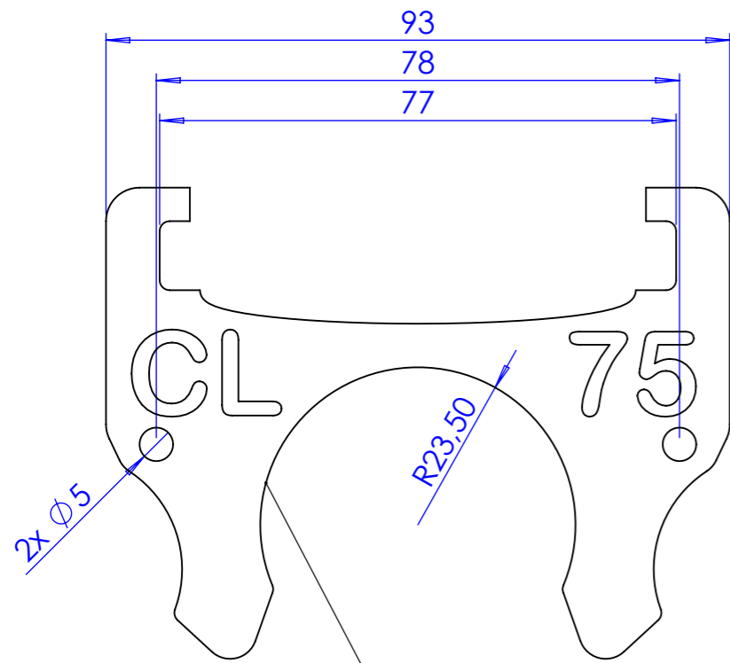
Clamp for pipe Ø48mm (1½")
