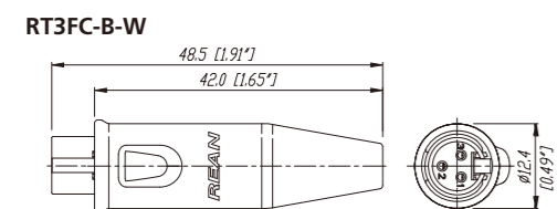
Female Pin Layout (Front)
