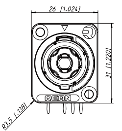
RLS4MDZ-H
