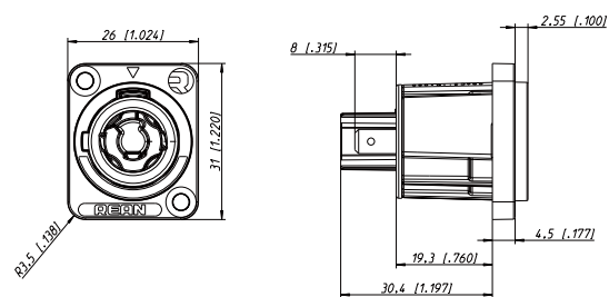
RRAC31-G / RRAC30-G
