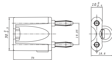
NYS5508-B
