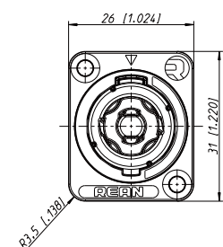
RLS4MDZ-H
