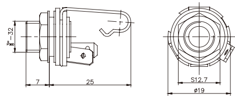
NYS229
