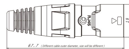
RCEM-Z-00*
