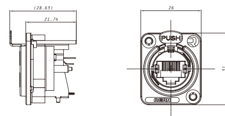
RRE8F-D-001
