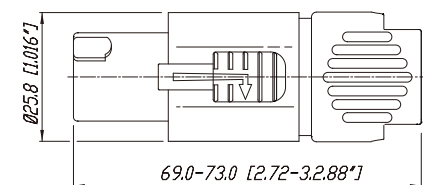
RLS4FC
