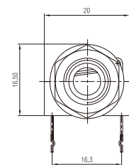
NYS219
