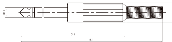
NYS204
