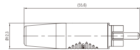
RF2C-*
