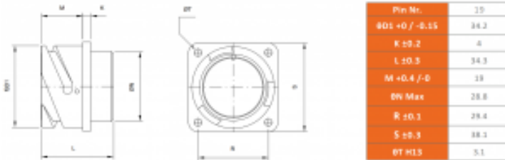
19 Way - Panel Receptacle Connector
