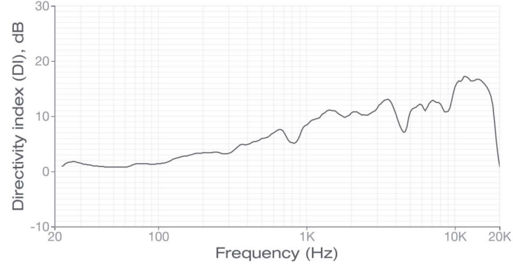
DIRECTIVITY INDEX
