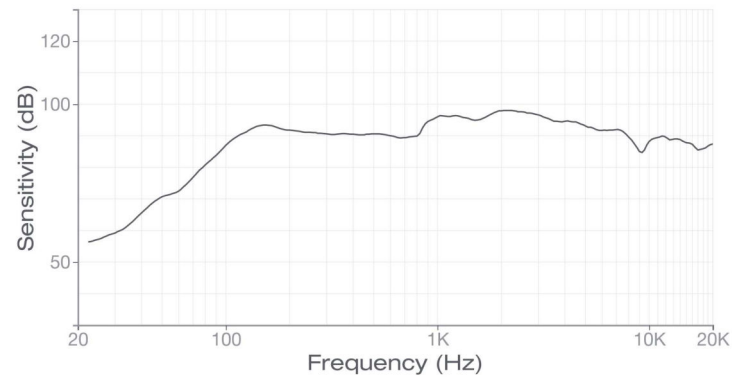
SENSITIVITY (SPL)
