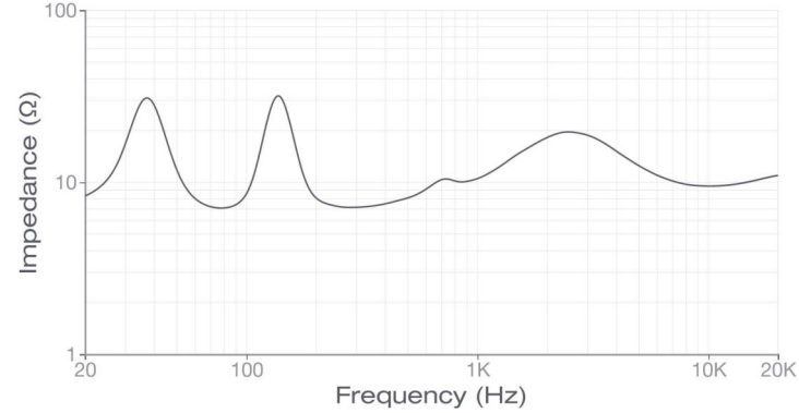
IMPEDANCE
