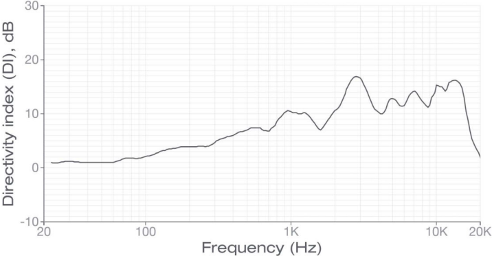
DIRECTIVITY INDEX
