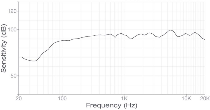
SENSITIVITY (SPL)
