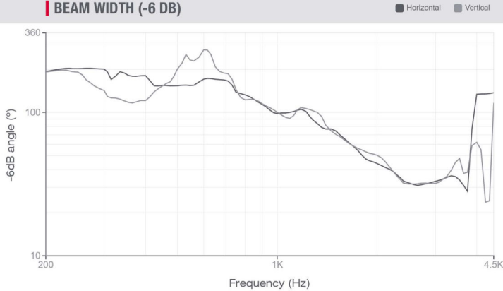
BEAM WIDTH (-6 DB)
