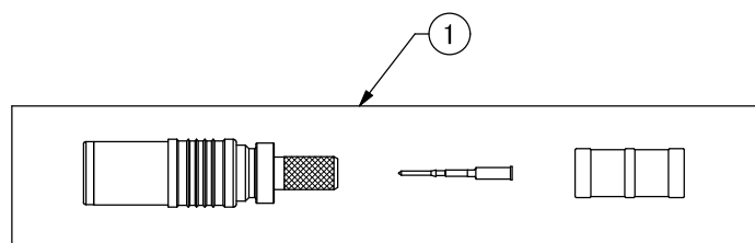
Connector Unit (DCP-C25HW-ML)
